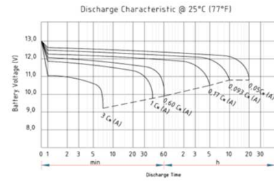
Duration of Discharge vs. Discharge Current
