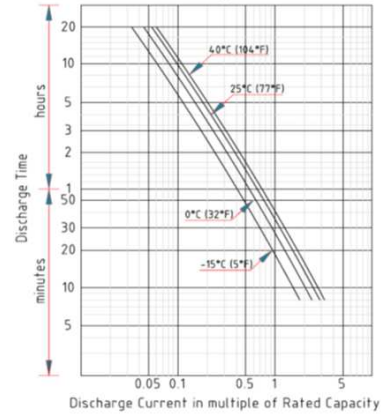
Duration of Discharge vs. Discharge Current
